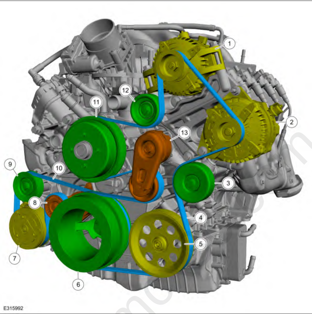
Accessory Drive Belt Routing “ With Dual generators
